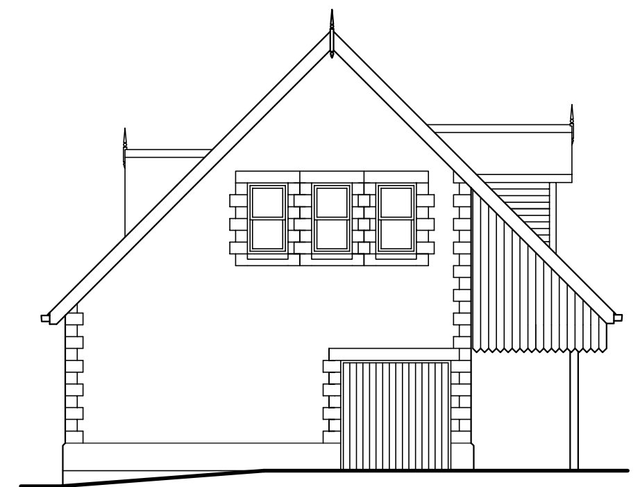
END ELEVATION: east
